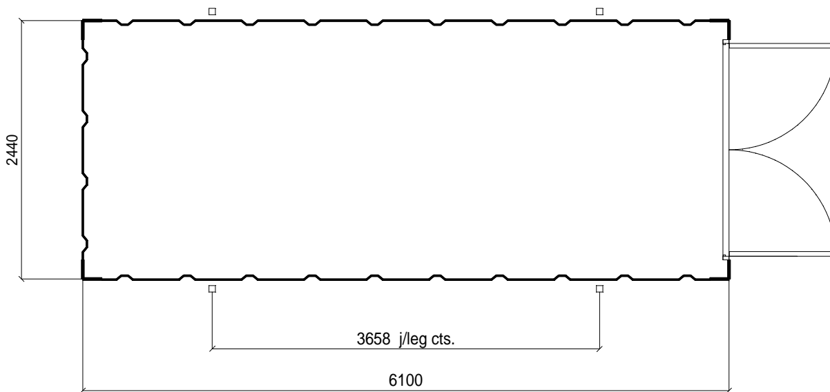
PLAN LAYOUT
