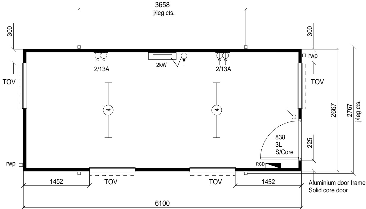
PLAN LAYOUT
