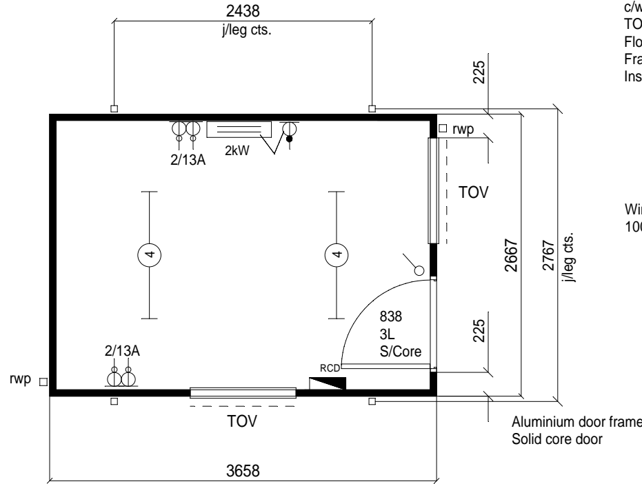
PLAN LAYOUT
