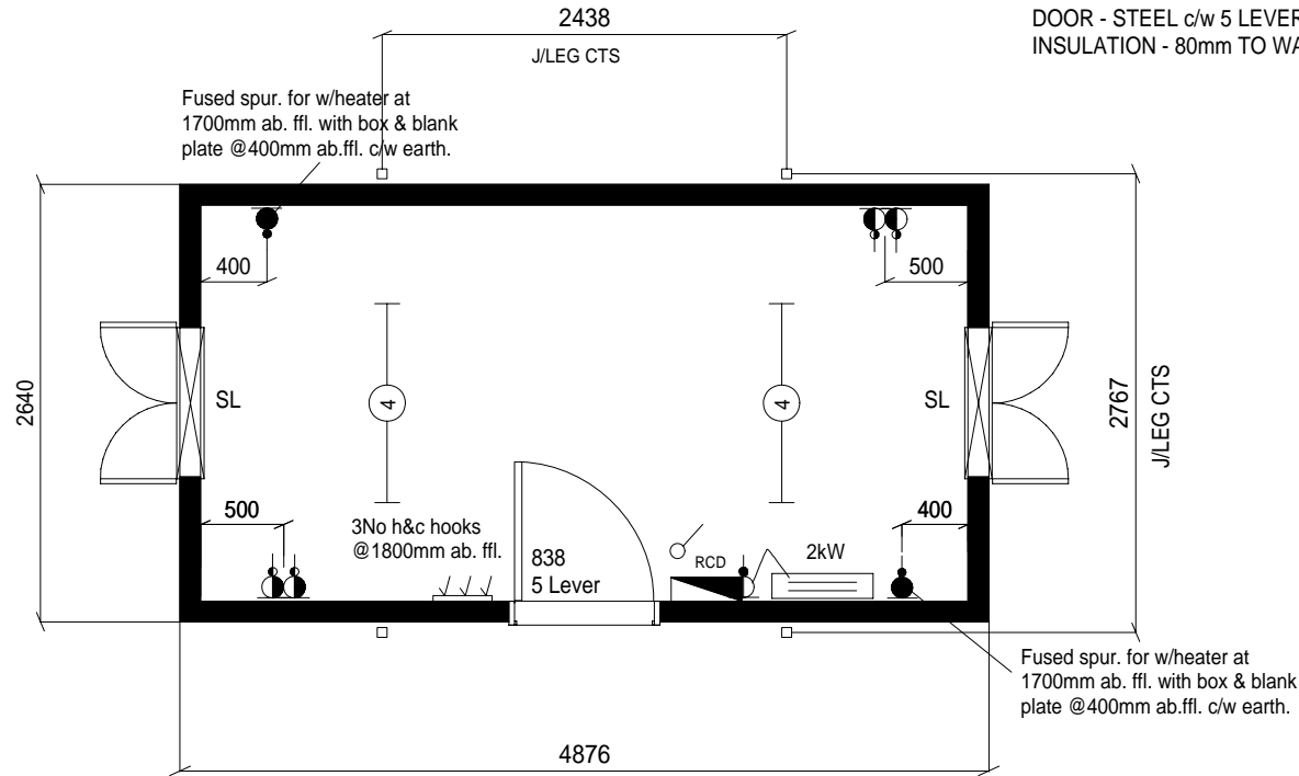
PLAN LAYOUT
